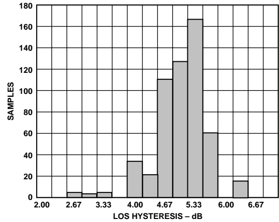
Figure 8. Histogram LOS Hysteresis 22.1 kΩ R_{THRESH} (All Temperature All Supply)
